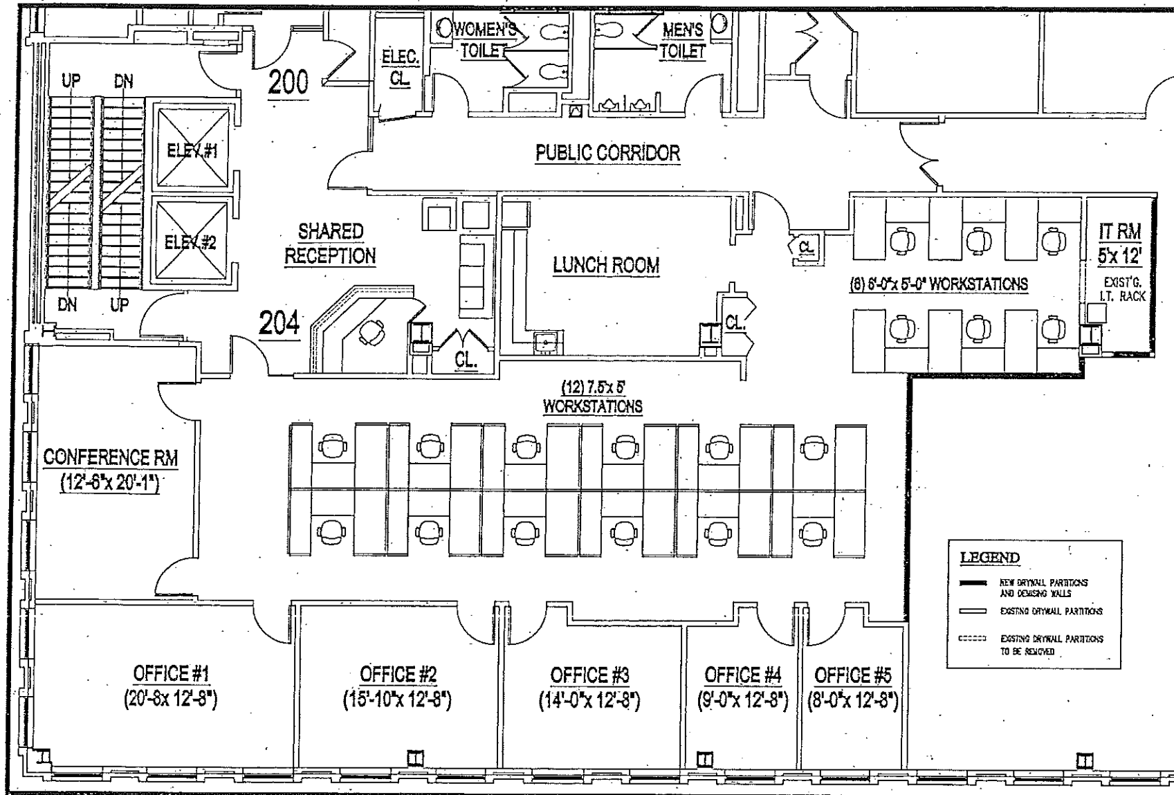
KEY PLAN
